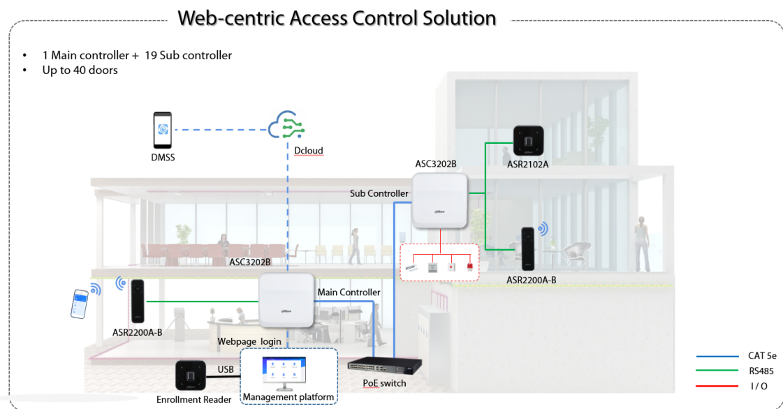
Figure 2-1 Networking diagram
