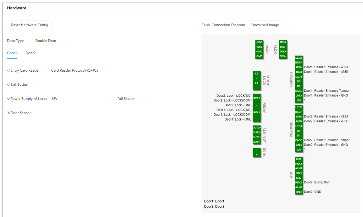
Figure 2-69 Hardware
