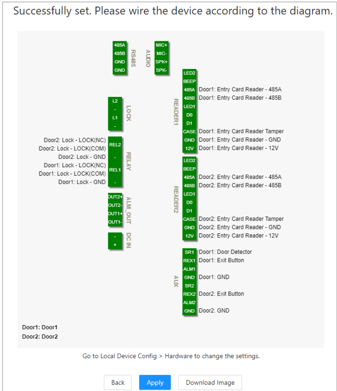
Figure 2-8 Wiring diagram
