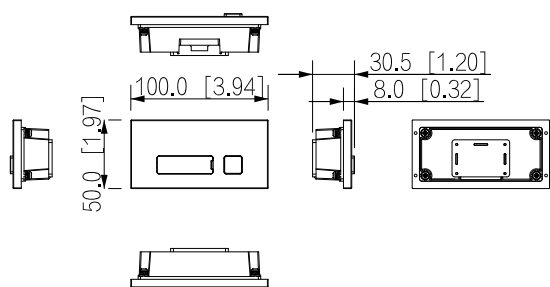
DHI-VTO4202F-MB1
