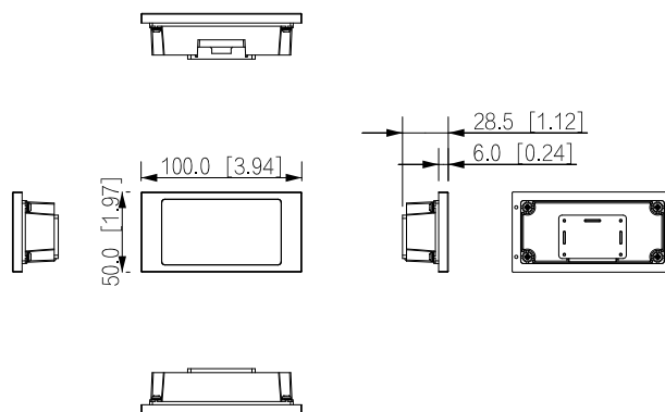
DHI-VTO4202FB-MR, DHI-VTO4202FB-MR1
