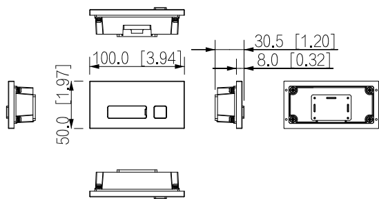
DHI-VTO4202FB-MB1
